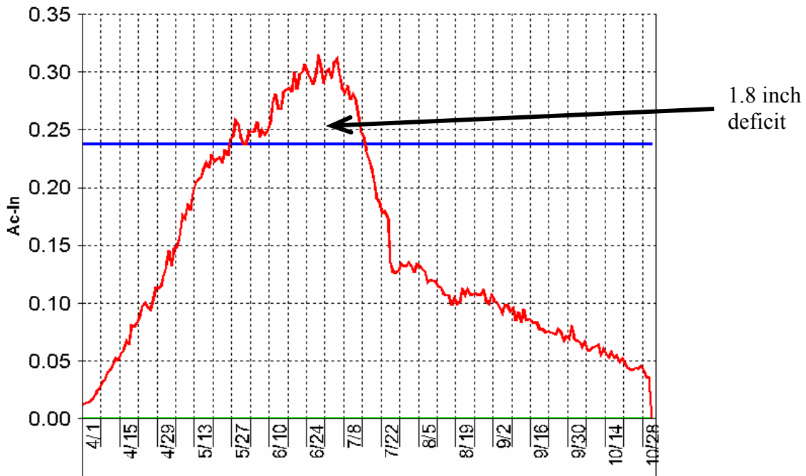
Figure 8. Seasonal ET and water supply for 65 ac spring grain and 65 ac alfalfa at Kimberly, ID, 80% irrigation water for season , wheel line.
