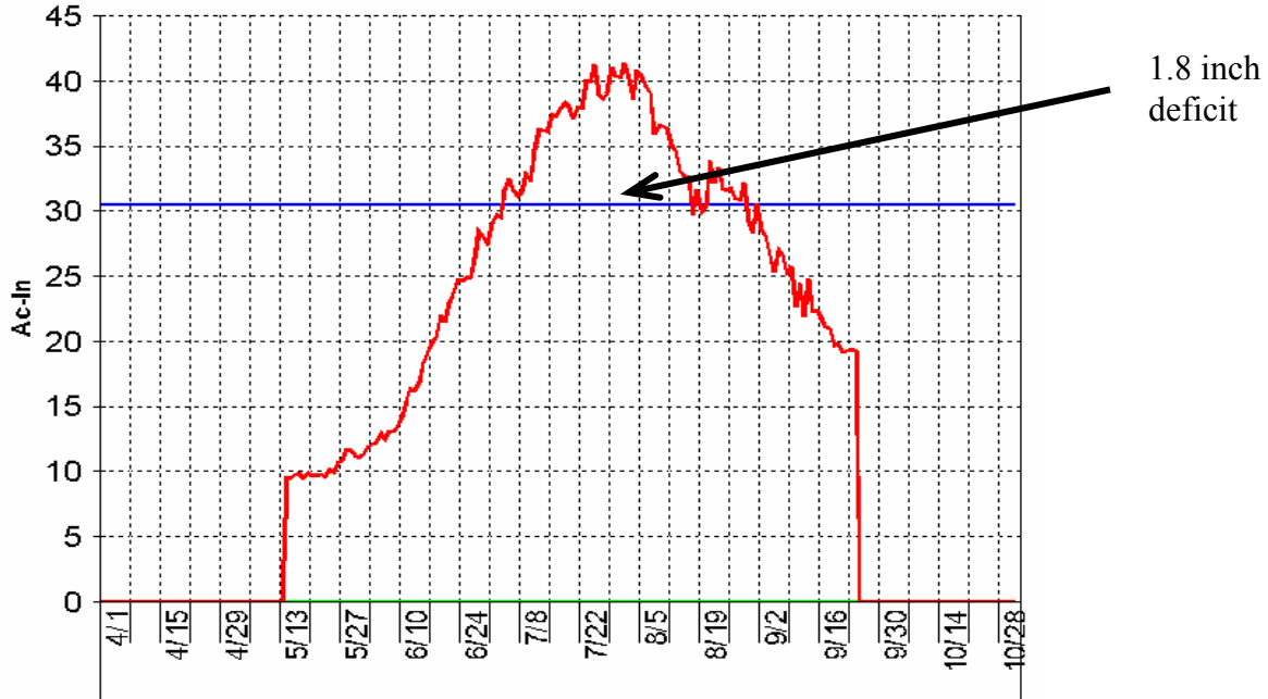
Figure 9. Seasonal ET and water supply for 130 acres of corn at Kimberly, ID, 80% irrigation water for season, pivot.
