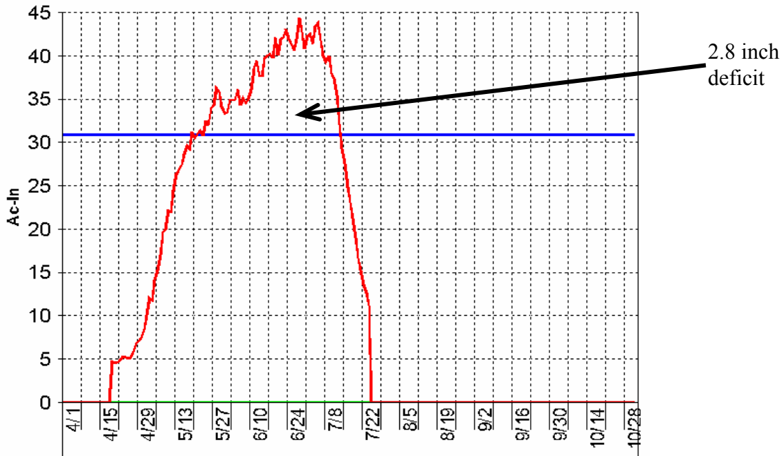
Figure 7. Seasonal ET and water supply for 130 acres of spring grain at Kimberly, ID, 80% irrigation water for season , wheel line.
