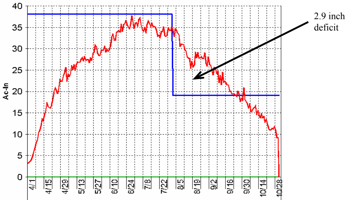
Figure 3. Seasonal ET and water supply for 130 acres of alfalfa at Kimberly, ID 8/1 cutback to 50% irrigation water.
