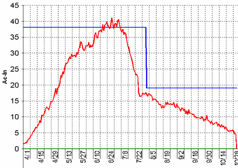
Figure 5. Seasonal ET and water supply for 65 ac spring grain and 65 ac alfalfa at Kimberly, ID, 8/1 cutback to 50% irrigation water.
