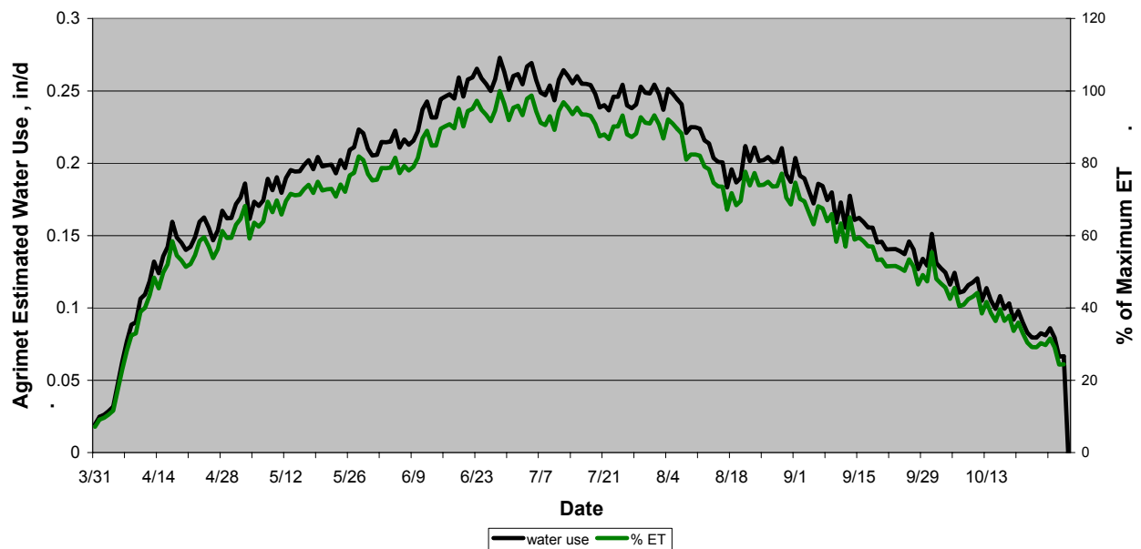
Figure 1. AGRIMET estimated water use in inches per day and % of maximum ET for Kimberly, ID. This figure can be used with lawns having a timer with a % ET setting. Enter the graph at the appropriate date, move up to intersect “% ET” line and read setting to meet ET on right axis.
