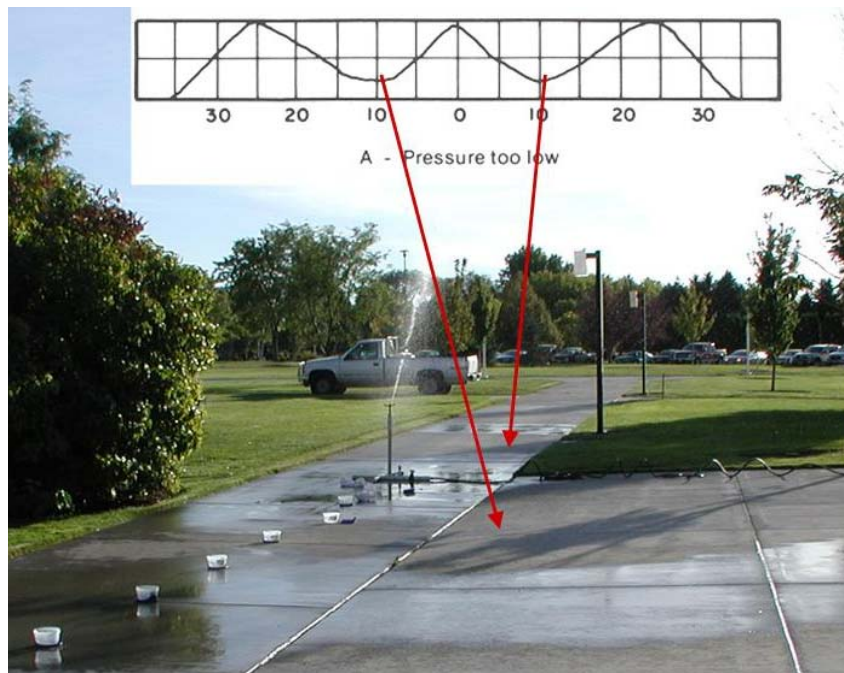
Figure 3. Water distribution from a sprinkler test using a brass nozzle at 20 psi system pressure for 20 minutes. Note the dry areas on the pavement corresponding to low areas in the theoretical distribution shown above.
