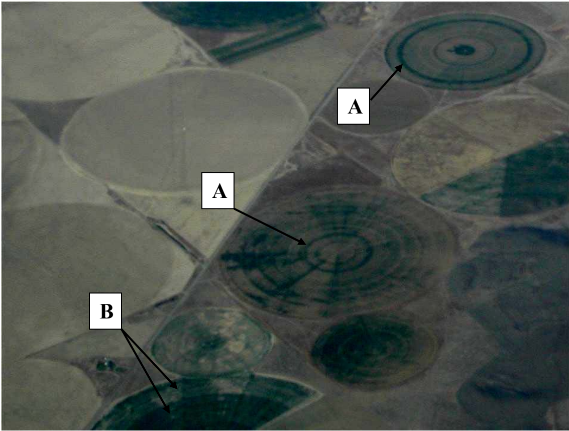
Figure 5. Poor center pivot uniformity due to malfunctioning pressure regulators (A) or incorrect nozzles on spans (B)
